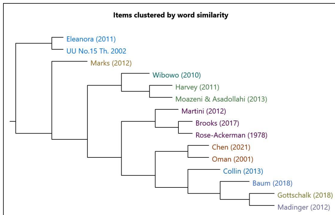
Figure 1. Cluster Analysis
